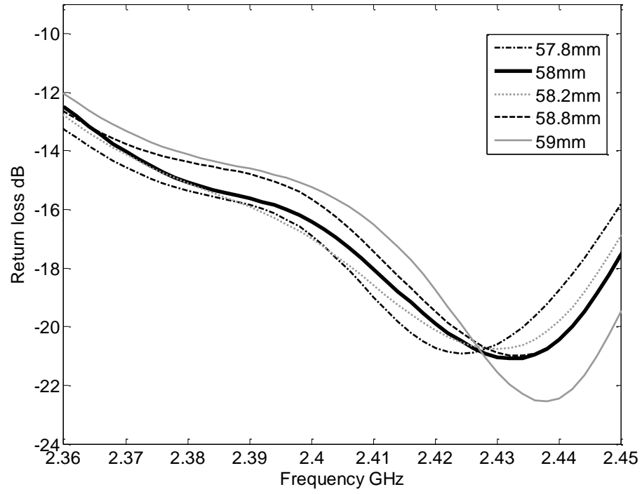
Figure 3-13 Return loss for ( L_r ) parametric study - proximity feeding
