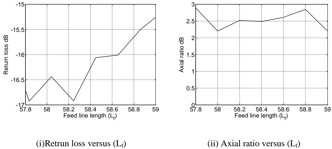
Figure 3-12 Parametric analysis of (L_f) at 2.4 GHz - proximity feeding
