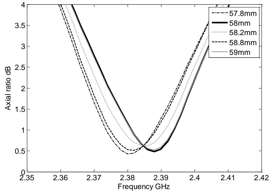
Figure 3-14 Axial ratio for ( L_r ) parametric study - proximity feeding
