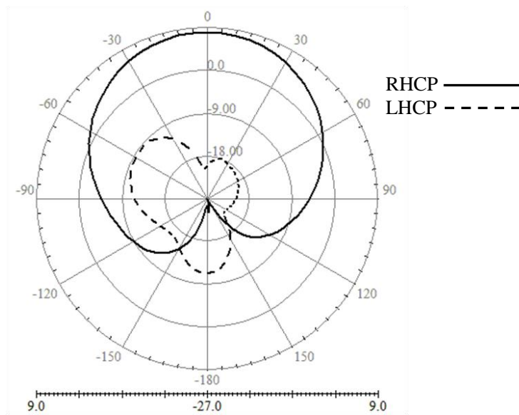
Figure 4-13 H-plane radiation pattern for proximity fed antenna @ f_r = 2.4\text{GHz}
