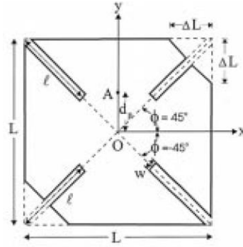
Figure 2-21 Truncated corner square microstrip antenna with 4 slits [4]
