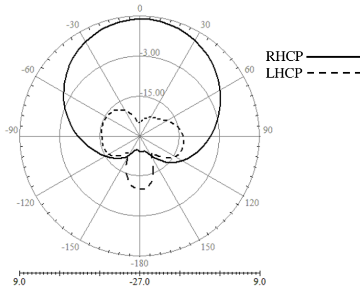
Figure 4-8 E-plane radiation pattern for microstrip line fed antenna @ f_r = 2.4\text{GHz}
